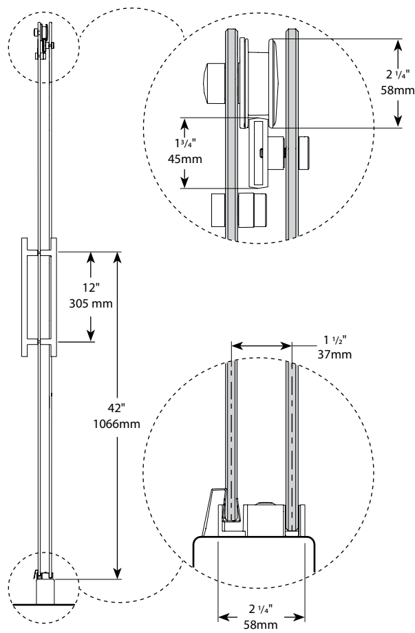
Suggested installation Installation proposée
